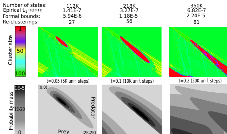
Fig. 1. Transient analysis of the Lotka-Volterra model using history-based adaptive aggregation.
